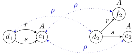
Figure 1: Two interpretations \mathcal{I}_1 and \mathcal{I}_2 and an \mathcal{ALCQ} bisimulation \rho , which is not an \mathcal{ALCQt} bisimulation.
