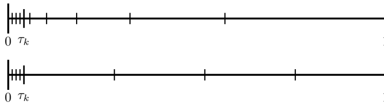
FIGURE 1. Shishkin mesh (below) and its variant with additional weak layer grading (top), \varepsilon_k = 10^{-2} , N = 8 , \beta = 1 , \sigma = 3 .
