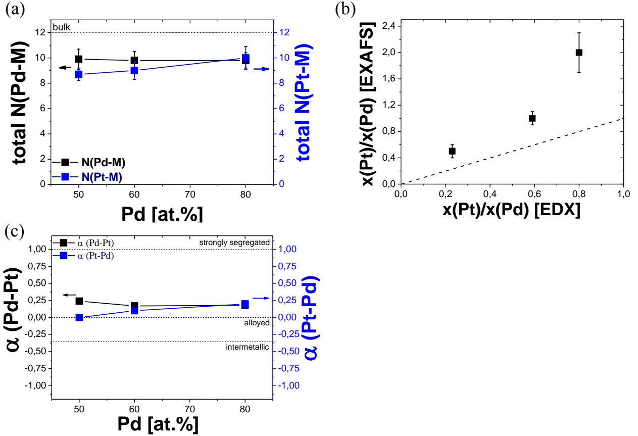
Figure 4. (a) Total coordination numbers ( N_{Pt-M} and N_{Pd-M} ) versus aerogel composition. (b) Chemical compositions obtained from EXAFS and EDX analysis. The dashed lines visualize the ideal mixture of bimetallic system. (c) Short range order parameter ( \alpha_{Pt-Pd} and \alpha_{Pd-Pt} ) in dependence of the content of Pd for the pristine Pd-Pt aerogels. Dashed lines symbolize the possible 3D-architectures of bimetallic systems such as intermetallic fcc motifs for \alpha = -1/3 , randomly disordered alloyed motifs for \alpha = 0 and strongly segregated motifs for \alpha = +1 .
