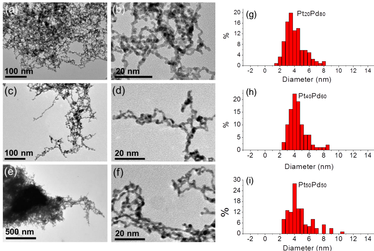
Figure 1. TEM micrographs of the \text{Pd}_{80}\text{Pt}_{20} (a, b), \text{Pd}_{60}\text{Pt}_{40} (c, d) and \text{Pd}_{50}\text{Pt}_{50} (e, f) aerogels at different magnifications. (g, h, i) Diagrams of the nanochain diameter distributions for each Pd-Pt aerogel were established by measuring of more than 100 regions of the nanochain segments. The mean diameters of the nanochains are 4.0 \pm 1.4 nm, 4.3 \pm 1.2 nm and 4.2 \pm 1.2 nm for the \text{Pd}_{80}\text{Pt}_{20} , \text{Pd}_{60}\text{Pt}_{40} and \text{Pd}_{50}\text{Pt}_{50} aerogels, respectively.
