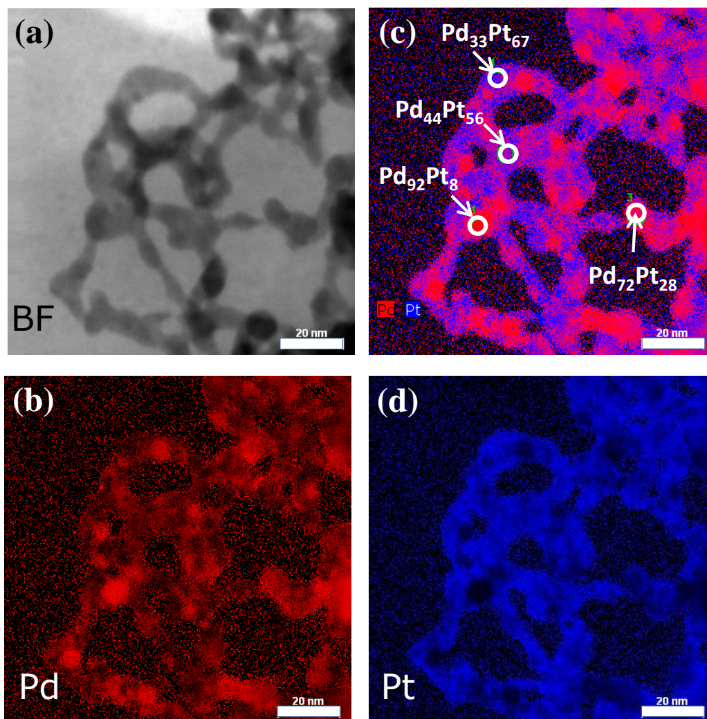
Figure 5. Bright-field STEM micrograph (a) and the corresponding EDX maps for the Pd (b) and Pt (d) measured from this region of the \text{Pd}_{50}\text{Pt}_{50} aerogel. (c) Overlap of the EDX maps for each element. The Pd and Pt are denoted with red and blue color, respectively. The scale bar is 20 nm.
